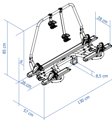
Thule Caravan Superb XT Black - Standard
