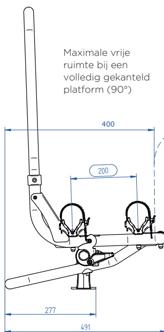
Thule Caravan Superb Short - 307329 Thule Caravan Superb XT Short - 302030
