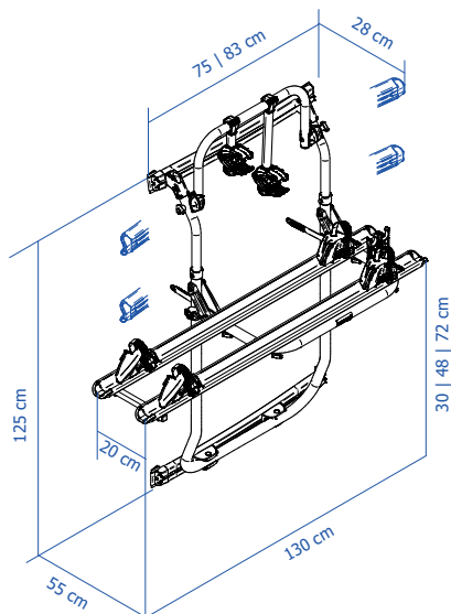
Thule Elite Van XT - Black VW Crafter ≥ 2017 (302018)
