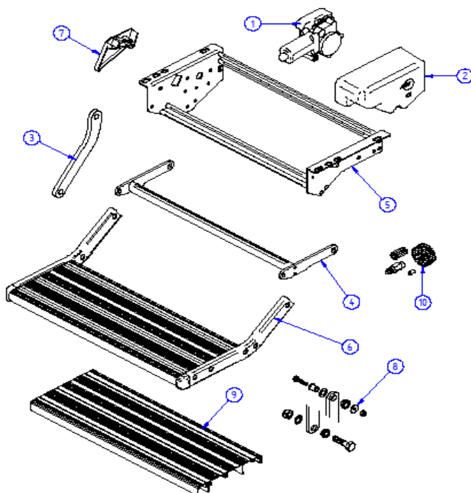
THULE Single step 12V ALU
