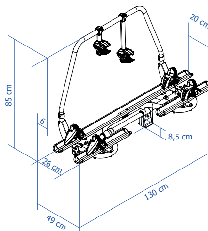
Thule Caravan Superb XT Black - Short
