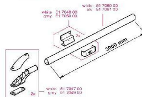
Thule Ladder – Roof Rack Deluxe
